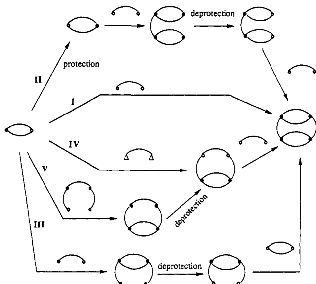
Figure 1. Synthetic strategies (I-V) for the construction of cylindrical macrotricyclic polyethers (○ = reactive sites; △ = epoxide ring which opens to give a reactive OH unit; • = protected or unreactive sites).
